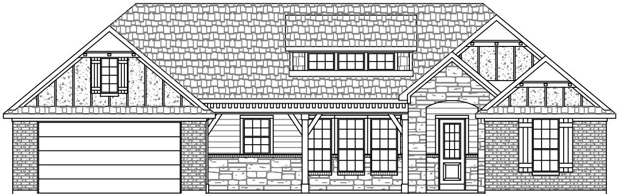
ELEVATION "B" 3-SIDES MASONRY
