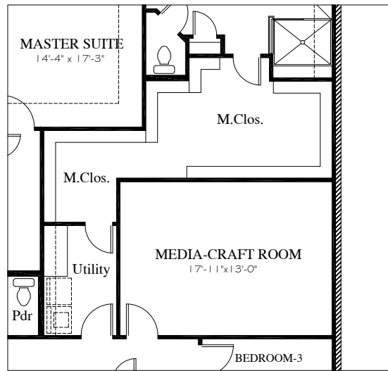
Media Room-Craft Room Option-2
