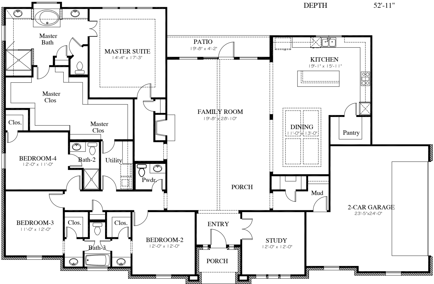
FLOOR PLAN
